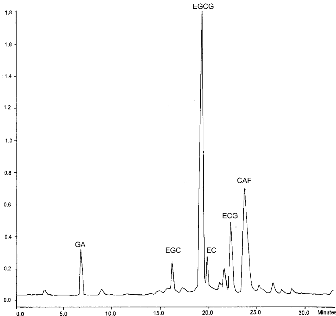
Figure 1. HPLC chromatogram of green tea at 280 nm. Peaks: GA, gallic acid; EGC, (-)-epigallocatechin; EGCG, (-)-epigallocatechin gallate; EC, (-)-epicatechin; ECG, (-)-epicatechin gallate; CAF, caffeine.
